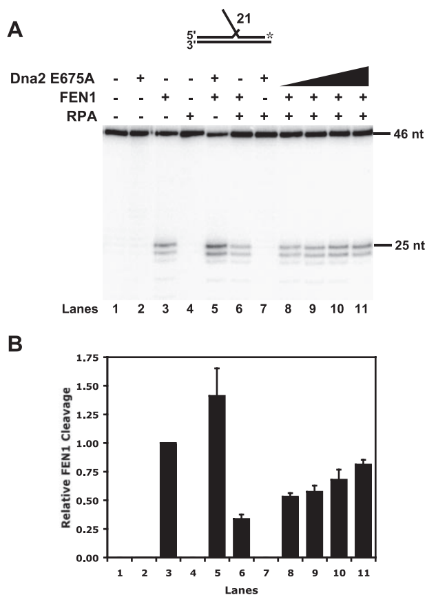
FIGURE 5. Dna2 E675A overcomes RPA inhibition of FEN1. RPA (200 fmol), FEN1 (0.25 fmol), and Dna2 E675A (10, 20, 100, and 200 fmol) were mixed followed by the addition of a 21-nt flap substrate (D7:U3:T3) (lanes 8–11). Denaturing PAGE was then used to separate the products. Lane 1 is the substrate alone control. Lanes 2–4 are substrate with Dna2 E675A (200 fmol), substrate with FEN1 (0.25 fmol), and substrate with RPA (200 fmol), respectively. Lanes 5–7 are substrate with Dna2 E675A (200 fmol) and FEN1 (0.25 fmol), substrate with RPA (200 fmol) and FEN1 (0.25 fmol), and substrate with Dna2 E675A (200 fmol) and RPA (200 fmol), respectively. B , graphical analysis of A . Each bar represents the conditions shown in the corresponding lane in A . The bars are an average of four independent experiments, and error bars represent the S.D. The substrate is depicted above the gel in A , and the asterisk indicates the site of the 3′- 32 P radiolabel.
