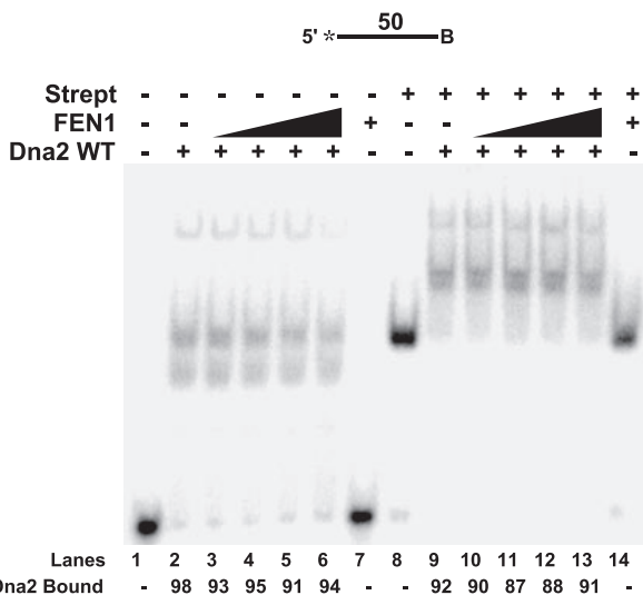
FIGURE 4. FEN1 cannot dissociate Dna2 on an ssDNA segment. A 50-nt ssDNA segment with a biotin attached at the 3'-end (D6) was used to test FEN1 disengagement of Dna2. In lanes 8–14 , streptavidin ( Strept ) was preincubated with the substrate. Dna2 (500 fmol) was bound to the ssDNA segment followed by the addition of FEN1 (5, 10, 25, and 50 fmol) ( lanes 3–6 and 10–13 ). Gel shift was then used to separate the products. Lanes 1, 2, and 6 are substrate alone, substrate with Dna2 (500 fmol), and substrate with FEN1 (50 fmol), respectively. Lanes 8, 9, and 14 are the same as lanes 1–3 , respectively, except with streptavidin. Percent Dna2 bound is defined as (Dna2 bound/(Dna2 bound + unbound substrate)) × 100. Substrates are depicted above gels, and the asterisk indicates the site of the 5'- 32 P radiolabel. WT , wild type. B indicates the site of biotin modification.
