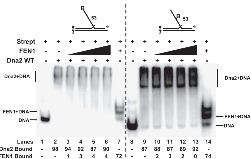
FIGURE 3. FEN1 requires its tracking mechanism to disengage flap-bound Dna2. Gel shift analysis was used to test Dna2 dissociation by FEN1 when tracking was blocked. Dna2 (500 fmol) was bound to a 53-nt flap substrate with a biotin attached at either the 5' flap end (D4:U2:T2) or in the middle of the flap (D5:U2:T2). Streptavidin ( Strept ) was then added to the reaction for conjugation with the biotin. Following conjugation, FEN1 (5, 10, 20, and 50 fmol) was added ( lanes 3–6 and 10–13 ). Lanes 1 and 8 are streptavidin-bound substrate alone. Lanes 2 and 9 are streptavidin-bound substrate plus Dna2 (500 fmol). Lanes 7 and 14 are streptavidin-bound substrate plus FEN1 (50 fmol). Percent Dna2 bound is defined as (Dna2 bound/(Dna2 bound + FEN1 bound + unbound substrate)) × 100. Percent FEN1 bound is defined as (FEN1 bound/(FEN1 bound + Dna2 bound + unbound substrate)) × 100. Substrates are depicted above gels, and the asterisk indicates the site of the 3'- 32 P radiolabel. WT , wild type. B indicates the site of biotin modification.
