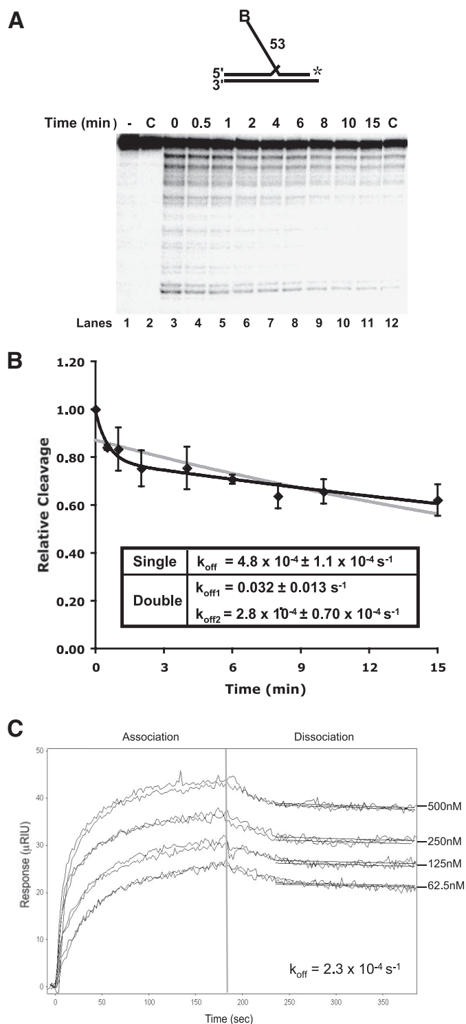
FIGURE 1. Slow dissociation of Dna2 from DNA substrates. A, Dna2 (200 fmol) and 5 fmol of a radiolabeled 53-nt flap substrate (D4:U2:T2) were incubated followed by the addition of 200-fold excess unlabeled flap substrate (D4:U2:T2). \text{MgCl}_2 was then added at the indicated time points. Dna2 cleavage was then measured by denaturing PAGE. Lane 1 is the substrate alone. Lane 2 is Dna2 with labeled and unlabeled substrate without \text{MgCl}_2 . In lane 12, the labeled and excess unlabeled substrates were mixed prior to the addition of Dna2. B, graphical analysis of A. Points were fit to a single (gray line) or double (black line) exponential decay curve using nonlinear least squares regression. Cleavage is defined as (cleaved/(cleaved + uncleaved)) \times 100 and values were then normalized to cleavage at time zero. For the double exponential decay curve, the dissociation amplitude described by the first curve was 21% and the second 78%. C, surface plasmon resonance was used to
