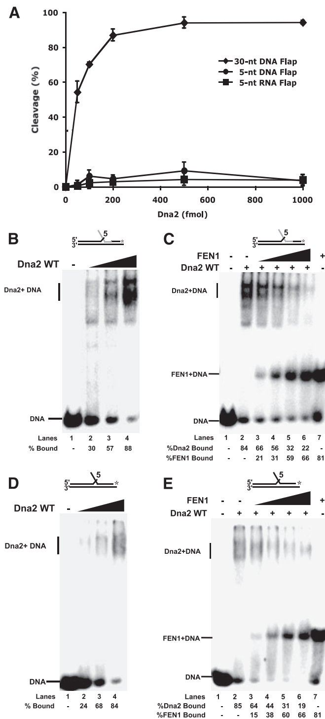
FIGURE 2. FEN1 disengagement of Dna2 from short RNA and DNA flaps to which Dna2 binds but cannot cleave. A , Dna2 (50, 100, 200, 500, and 1000 fmol) was incubated with 5 fmol of a 5-nt RNA flap substrate (D1:U1:T1) (squares), a 5-nt DNA flap substrate (D2:U2:T2) (circles), or a 30-nt DNA flap substrate (D3:U2:T2) (diamonds). Cleavage activity was then measured by denaturing PAGE. B , gel shift analysis was used to measure Dna2 (0.2, 0.5, 1 pmol) binding activity on the 5-nt RNA flap (lanes 2–4). Lane 1 is the substrate alone control. C , Dna2 (1 pmol) was pre-bound to the 5-nt RNA flap substrate followed by the addition of FEN1 (5, 10, 25, and 50 fmol) (lanes 3–6). The samples were then analyzed by gel shift. Lanes 1 and 7 are the substrate alone and substrate plus FEN1 (50 fmol), respectively. WT , wild type. D , as described in B , except a 5-nt DNA flap was used. E , as described in C , except a 5-nt DNA flap substrate was used. A , points are an average of three experiments, and the bars indicate the standard deviation. Percent cleavage is defined as (cleaved/(cleaved + uncleaved)) \times 100. Percent Dna2 bound is defined as
